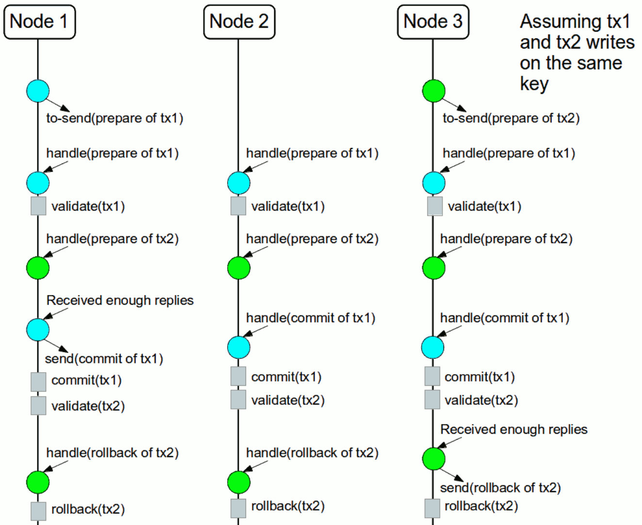
Figure 4. 2-phase commit
