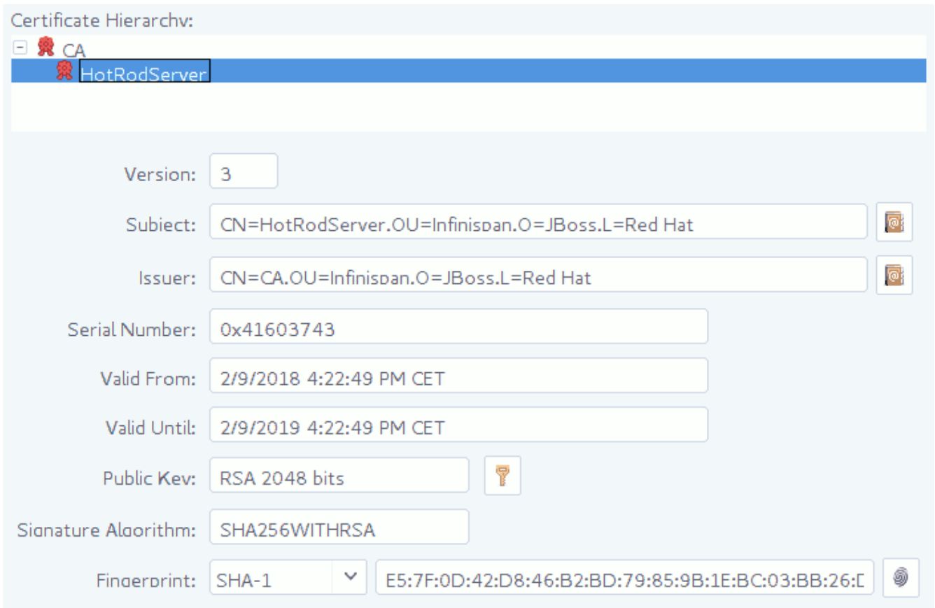
Figure 1. Certificate chain
