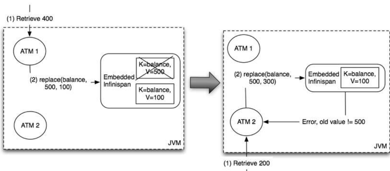
Figure 3. P2P solution
