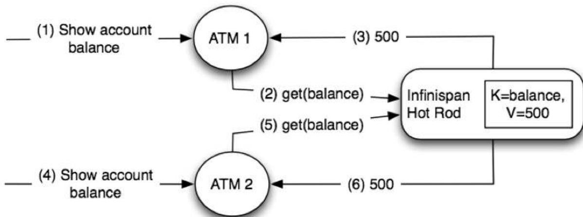
Figure 2. Concurrent readers
