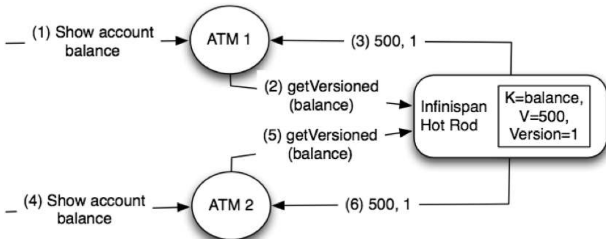
Figure 4. Get versioned
