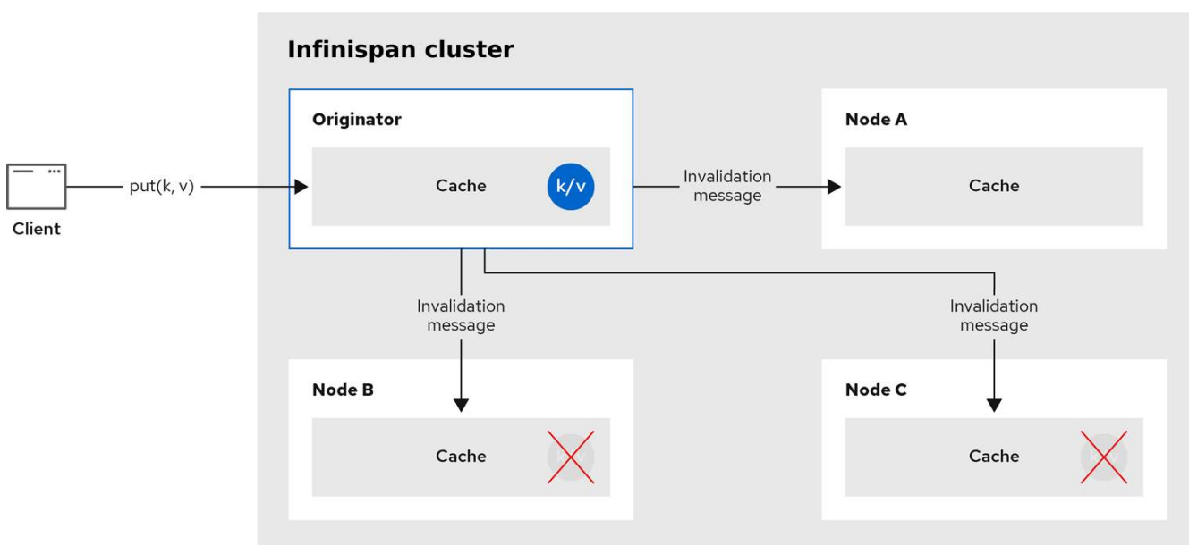
Figure 5. Invalidation cache
