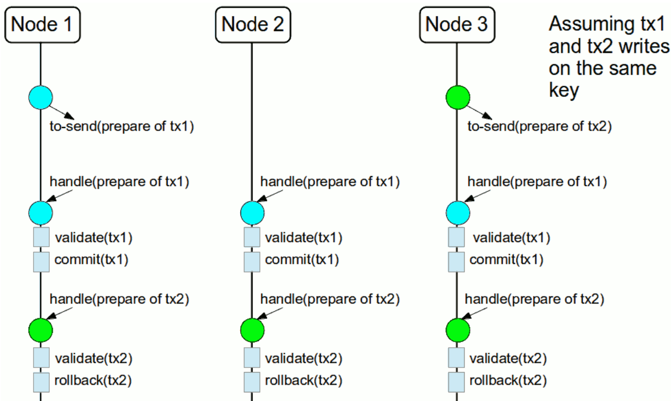
Figure 8. 1-phase commit
