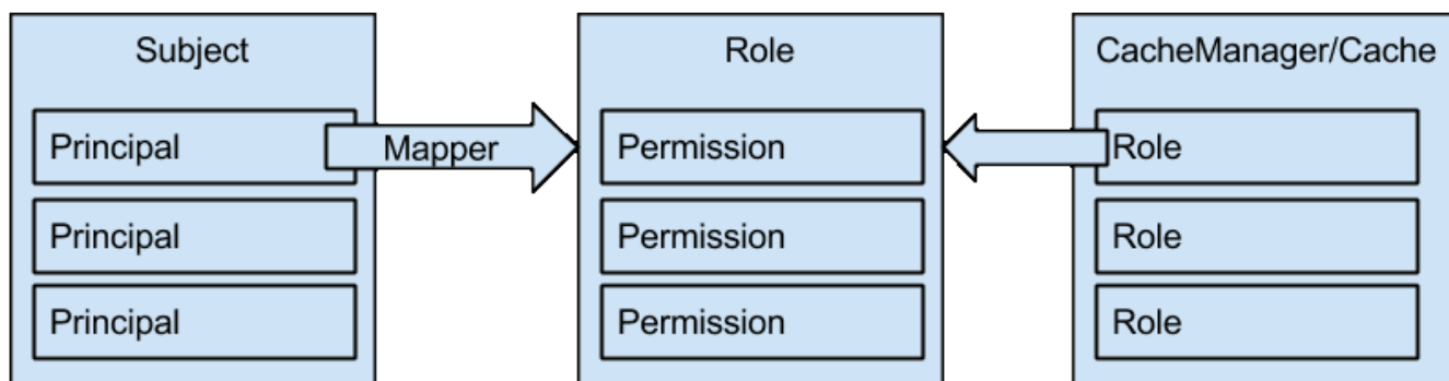
Figure 21. Roles/Permissions mapping
