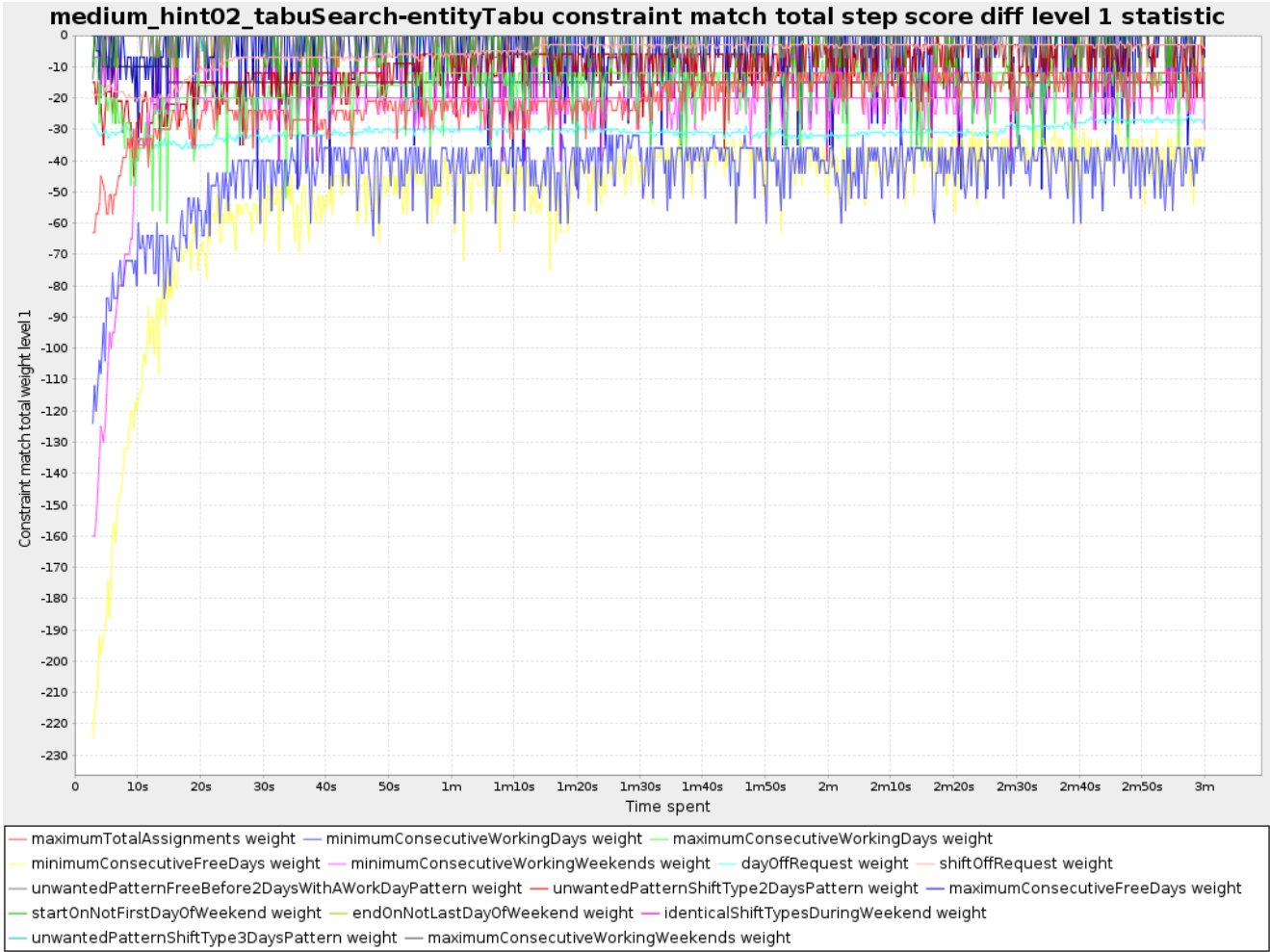
Figure 13.9. Constraint match total step score diff over time statistic
