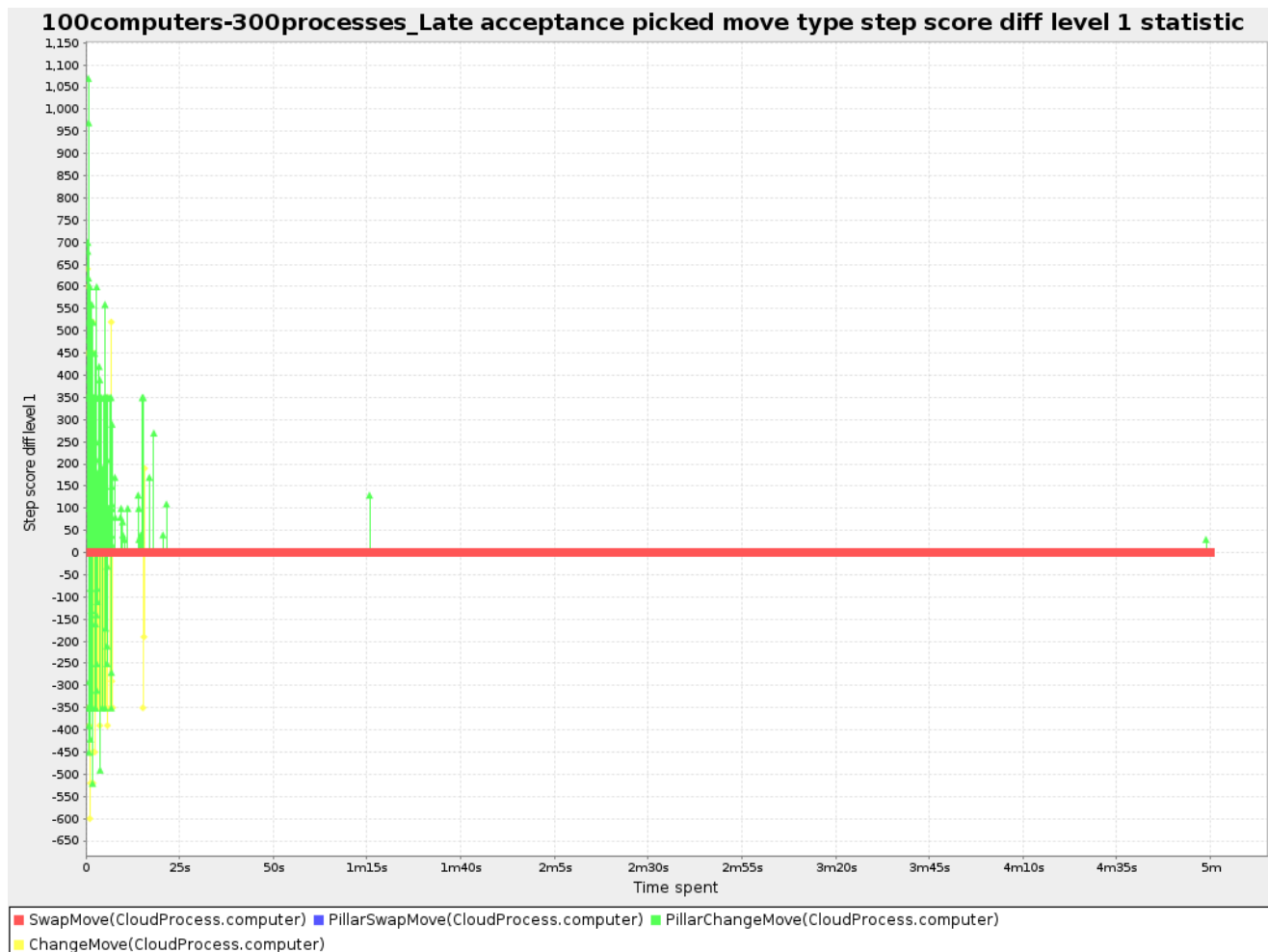
Figure 13.11. Picked move type step score diff over time statistic
