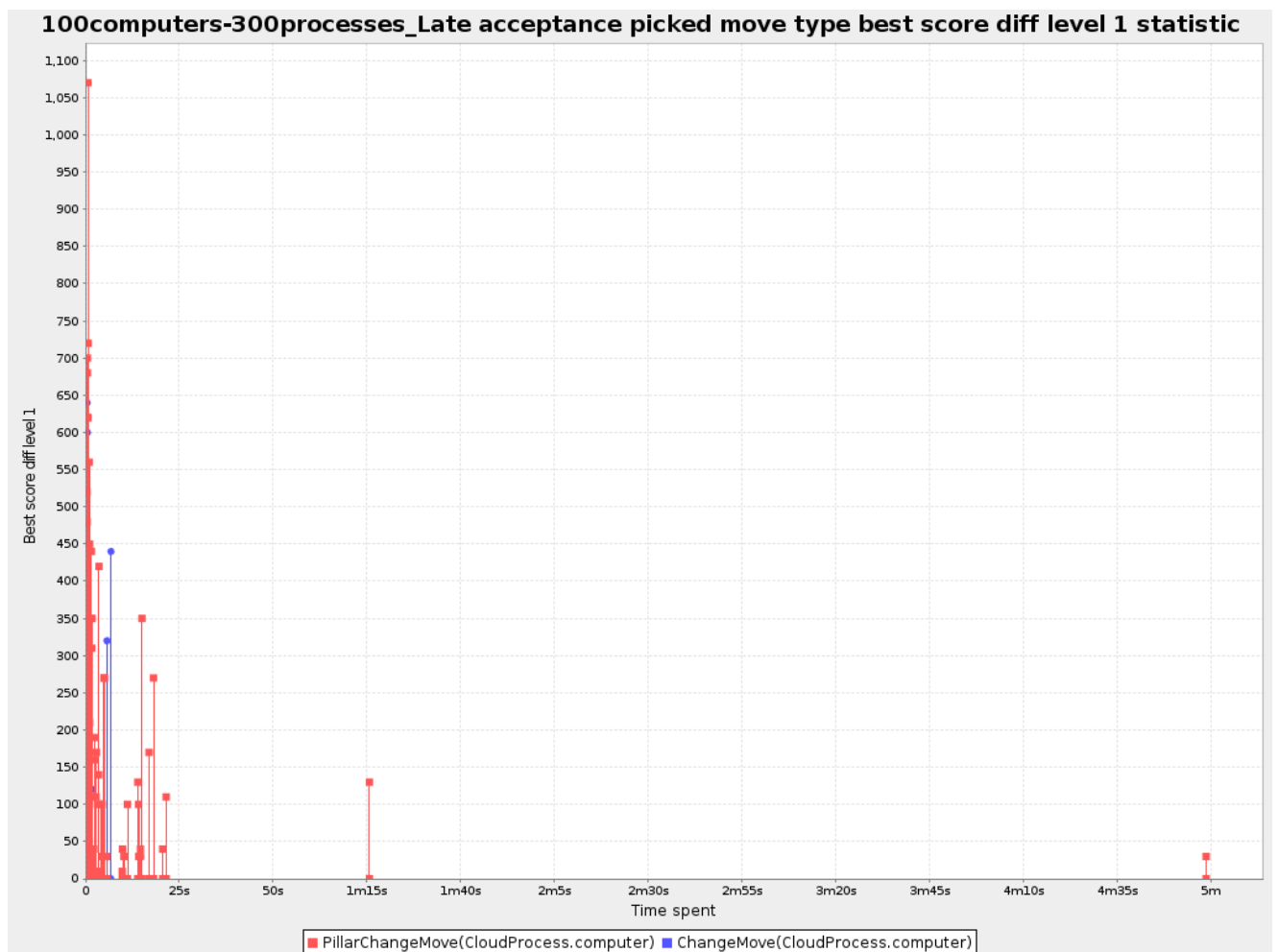
Figure 13.10. Picked move type best score diff over time statistic
