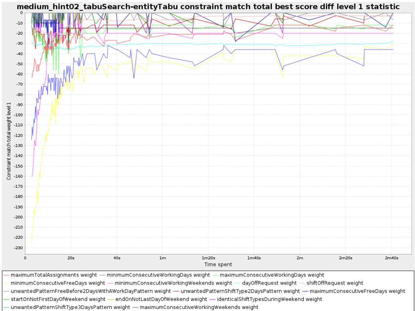
Figure 13.8. Constraint match total best score diff over time statistic
